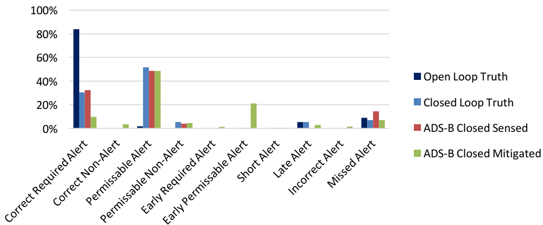
Figure 38. ADS-B Corrective Alert Scoring for NAS-Derived Uncorrelated Encounters
