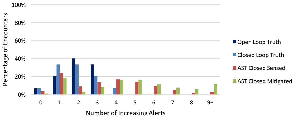
Figure 95. AST Alert Jitter for Overtake MOPS Requirement-Derived Test Vectors
