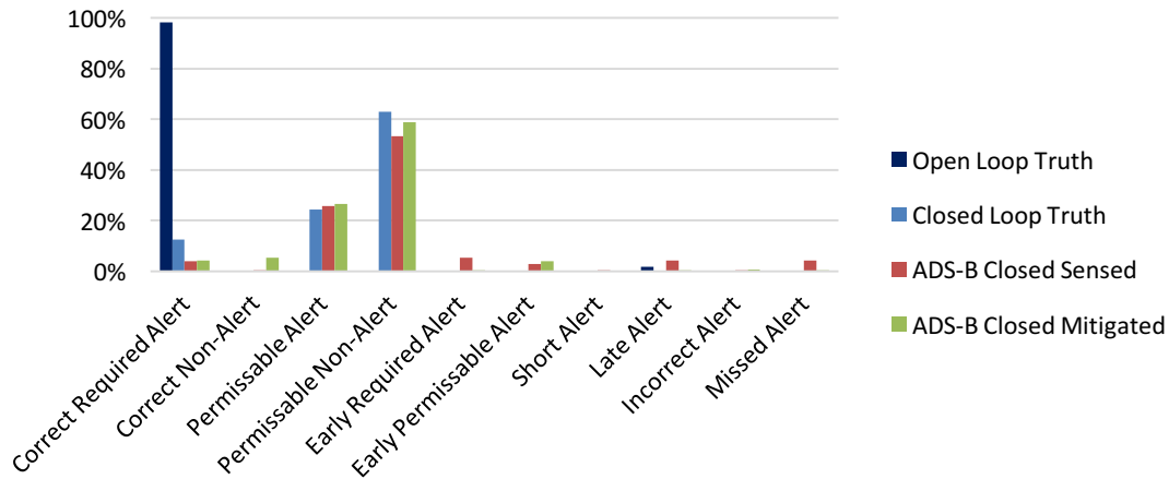
Figure 29. ADS-B Warning Alert Scoring for NAS-Derived Correlated Encounters
