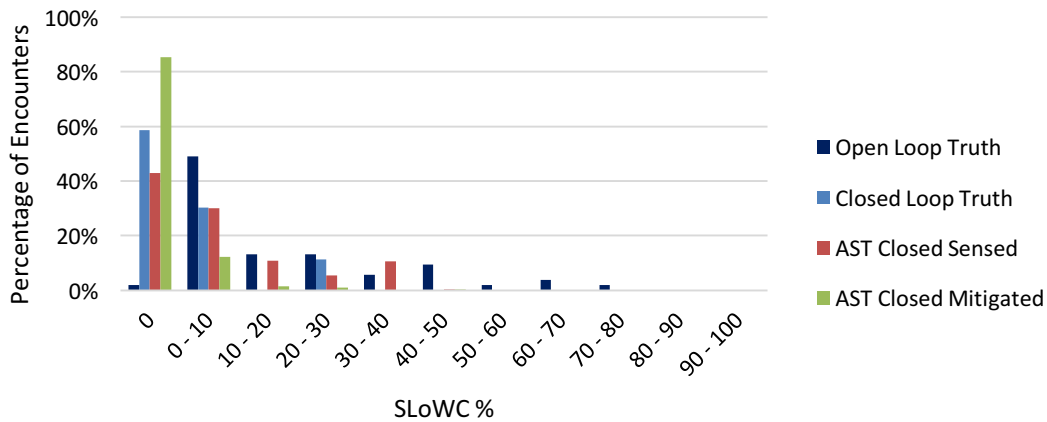
Figure 34. AST SLoWC for NAS-Derived Uncorrelated Encounters
