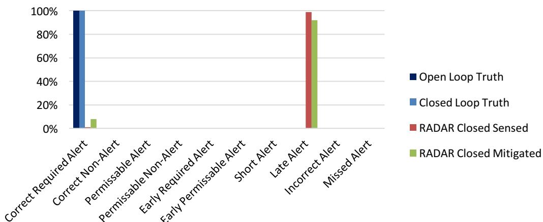
Figure 75. Radar Warning Alert Scoring for Maneuvering MOPS Requirement-Derived Test Vectors
