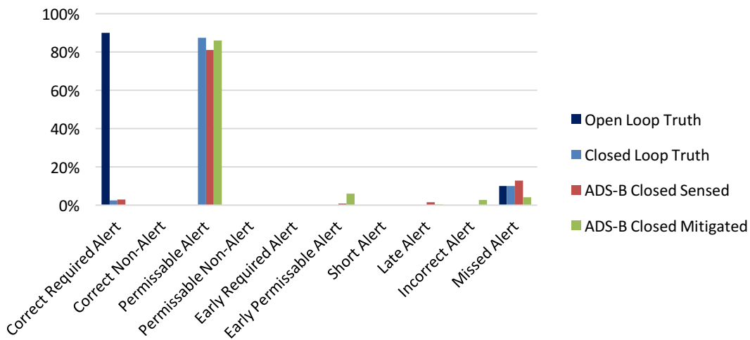
Figure 26. ADS-B Corrective Alert Scoring for NAS-Derived Correlated Encounters
