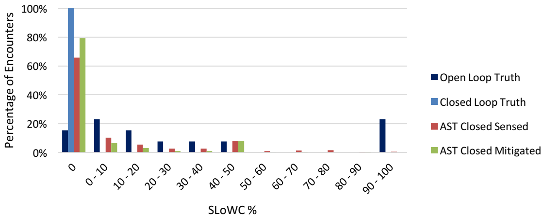
Figure 50. AST SLoWC for Converging MOPS Requirement-Derived Test Vectors
