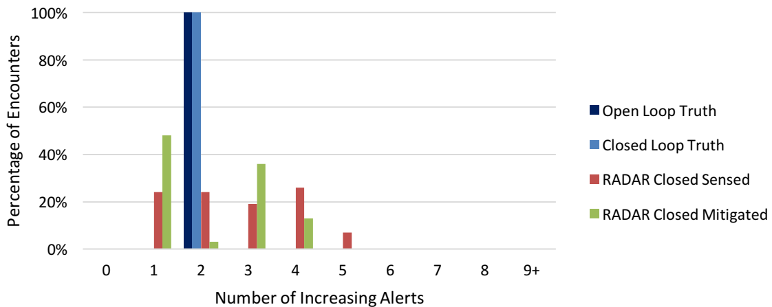
Figure 89. Radar Alert Jitter for Maneuvering MOPS Requirement-Derived Test Vectors
