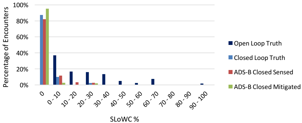
Figure 23. ADS-B SLoWC for NAS-Derived Correlated Encounters
