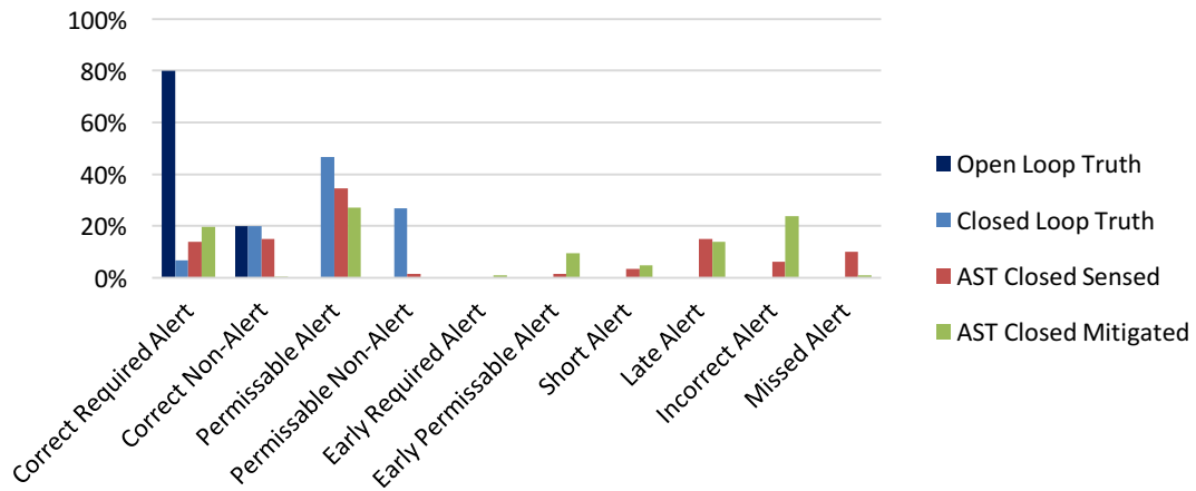
Figure 81. AST Warning Alert Scoring for Overtake MOPS Requirement-Derived Test Vectors
