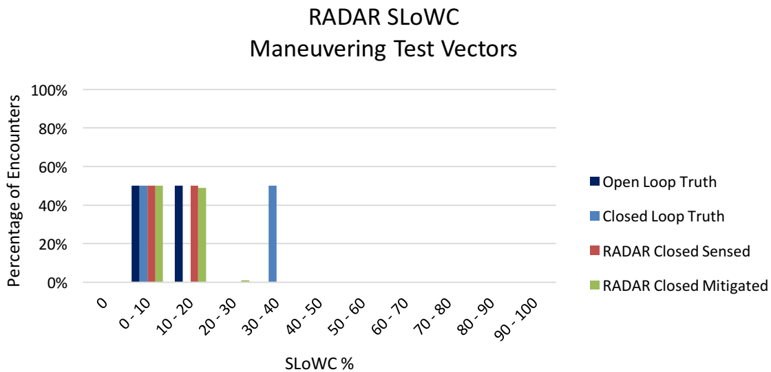
Figure 47. Radar SLoWC for Maneuvering MOPS Requirement-Derived Test Vectors
