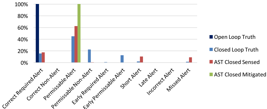
Figure 65. AST Corrective Alert Scoring for High Speed MOPS Requirement-Derived Test Vectors
