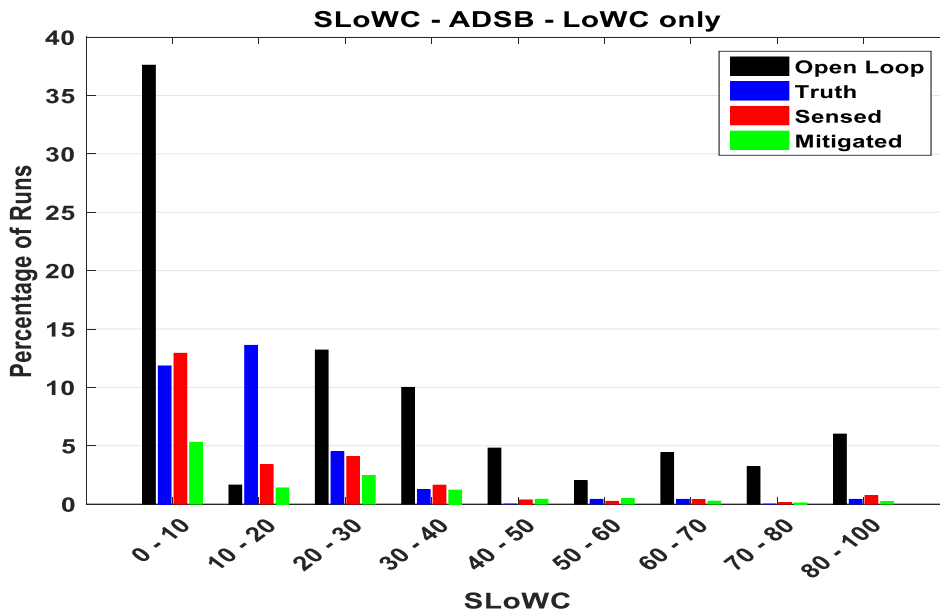
Figure 11. ADS-B SLoWC for Combined Encounters that Lost Well Clear
