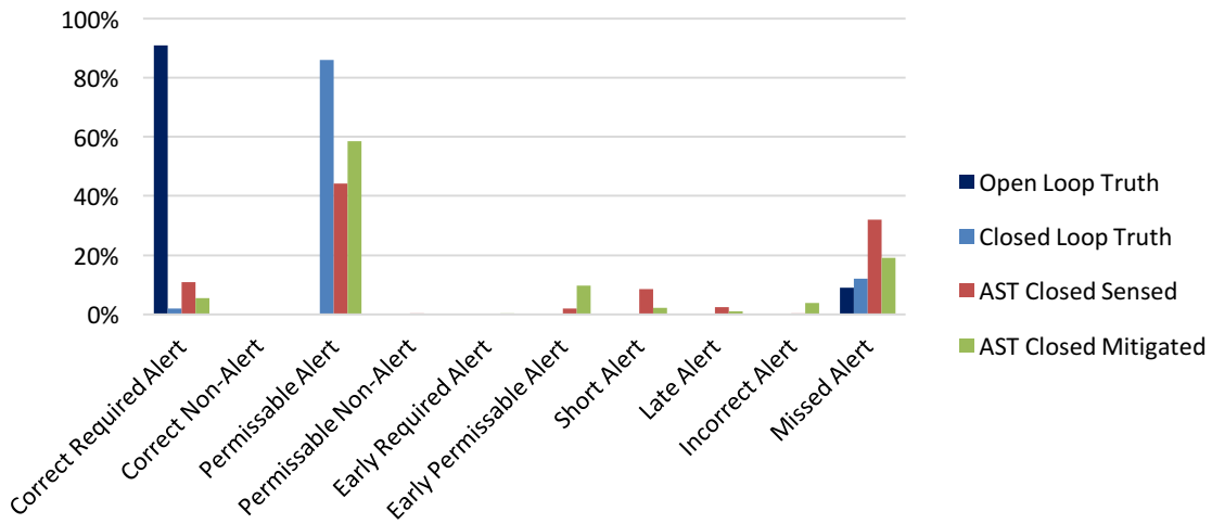
Figure 25. AST Corrective Alert Scoring for NAS-Derived Correlated Encounters
