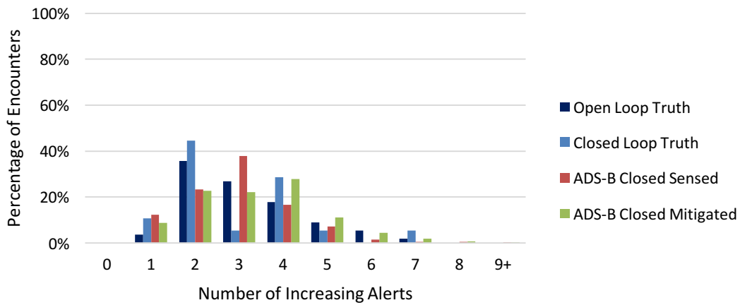
Figure 44. ADS-B Alert Jitter for NAS-Derived Uncorrelated Encounters
