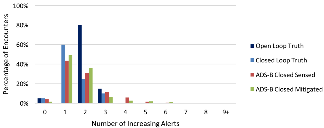
Figure 97. ADS-B Alert Jitter for Converging MOPS Requirement-Derived Test Vectors
