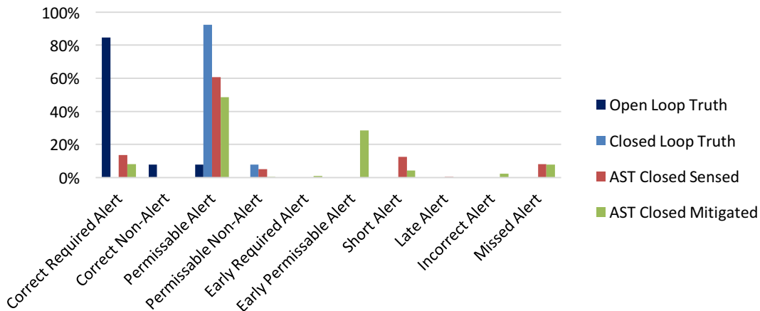
Figure 78. AST Warning Alert Scoring for Converging MOPS Requirement-Derived Test Vectors
