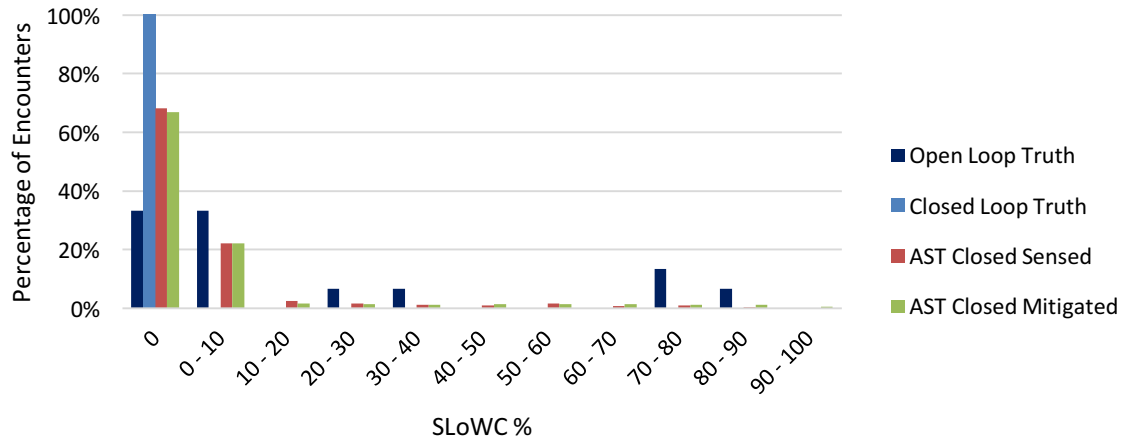
Figure 53. AST SLoWC for Overtake MOPS Requirement-Derived Test Vectors
