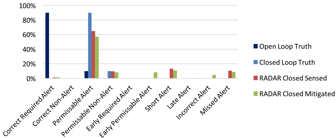
Figure 60. Radar Corrective Alert Scoring for Converging MOPS Requirement-Derived Test Vectors
