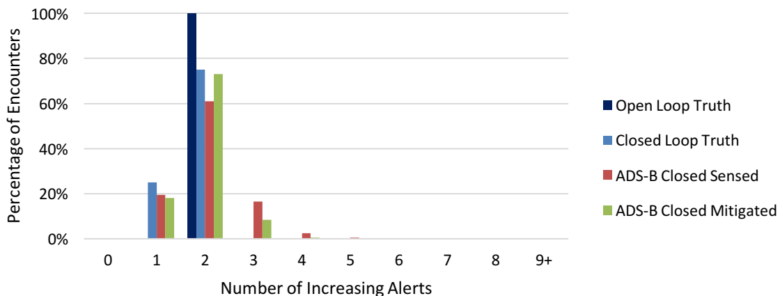
Figure 98. ADS-B Alert Jitter for High Speed MOPS Requirement-Derived Test Vectors
