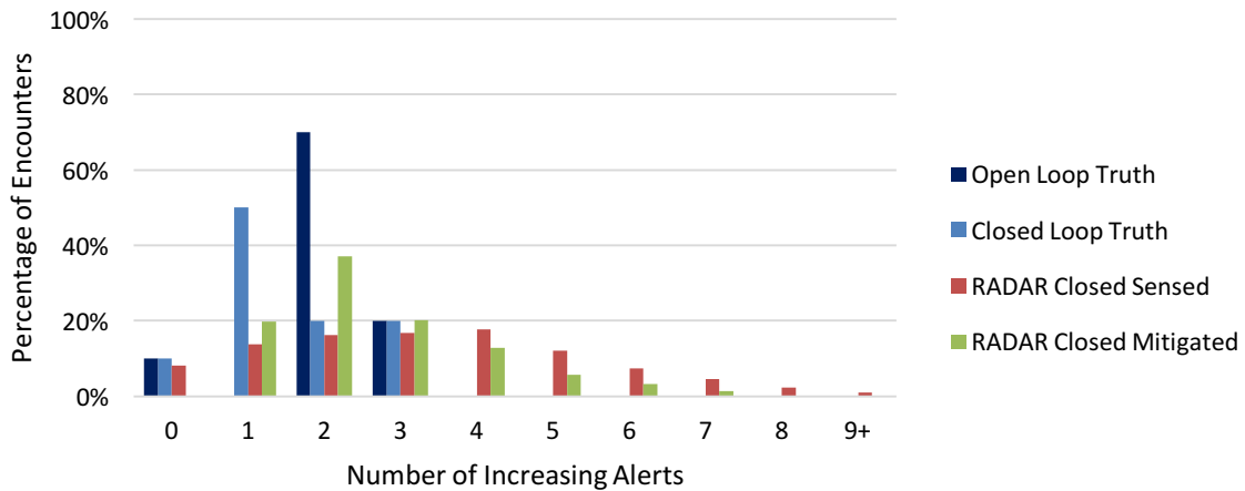
Figure 88. Radar Alert Jitter for Converging MOPS Requirement-Derived Test Vectors
