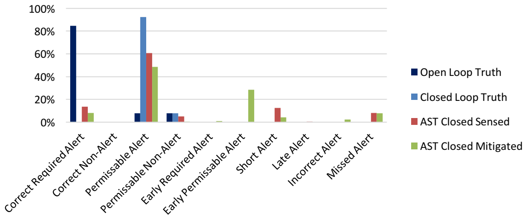
Figure 64. AST Corrective Alert Scoring for Converging MOPS Requirement-Derived Test Vectors
