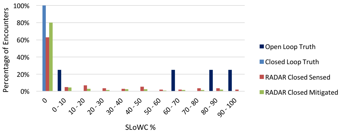
Figure 51. AST SLoWC for High-Speed MOPS Requirement-Derived Test Vectors
