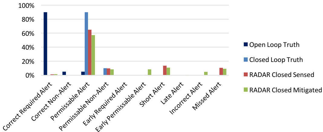
Figure 74. Radar Warning Alert Scoring for Converging MOPS Requirement-Derived Test Vectors
