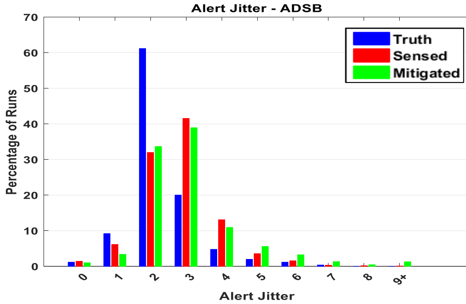
Figure 20. Open Loop ADS-B Alert Jitter for Combined Encounters
