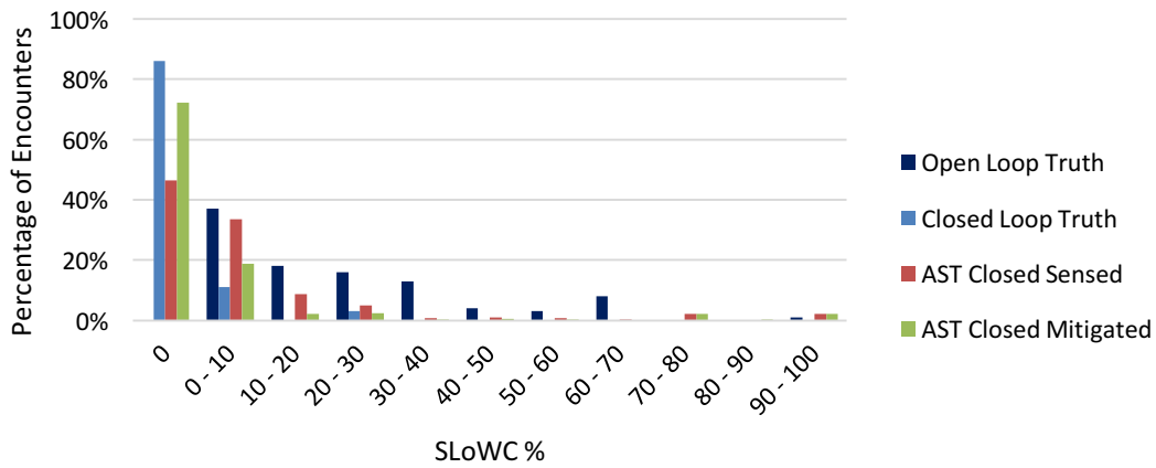
Figure 22. AST SLoWC for NAS-Derived Correlated Encounters
