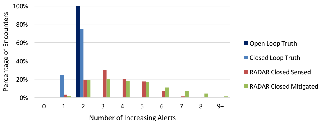
Figure 93. AST Alert Jitter for High Speed MOPS Requirement-Derived Test Vectors
