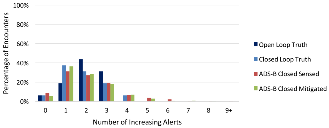
Figure 100. ADS-B Alert Jitter for Overtake MOPS Requirement-Derived Test Vectors
