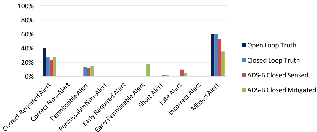
Figure 71. ADS-B Corrective Alert Scoring for Maneuvering MOPS Requirement-Derived Test Vectors
