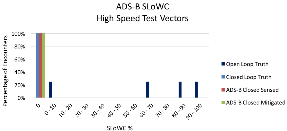
Figure 56. ADS-B SLoWC for High Speed MOPS Requirement-Derived Test Vectors
