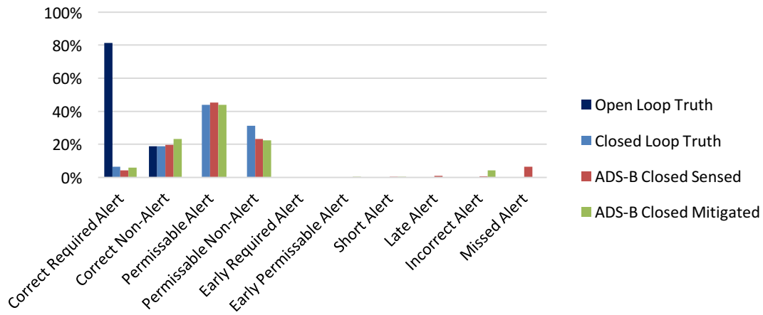
Figure 86. ADS-B Warning Alert Scoring for Overtake MOPS Requirement-Derived Test Vectors
