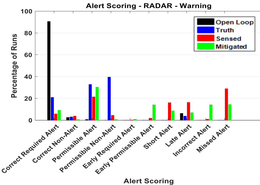
Figure 15. Radar Warning Alert Scoring for Combined Encounters
