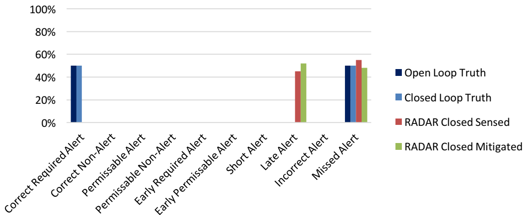
Figure 61. Radar Corrective Alert Scoring for Maneuvering MOPS Requirement-Derived Test Vectors
