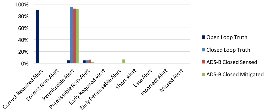
Figure 69. ADS-B Corrective Alert Scoring for Converging MOPS Requirement-Derived Test Vectors
