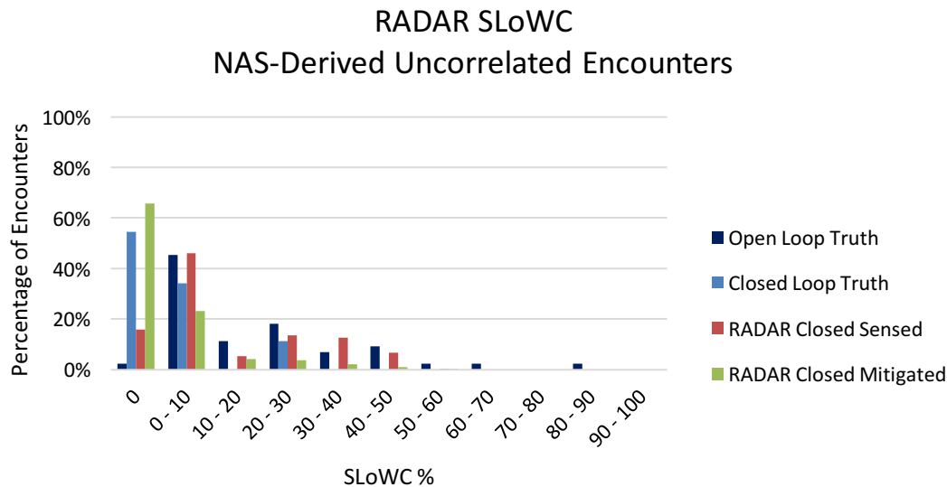
Figure 33. Radar SLoWC for NAS-Derived Uncorrelated Encounters
