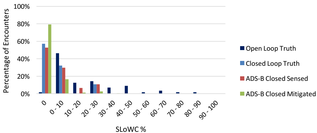
Figure 35. ADS-B SLoWC for NAS-Derived Uncorrelated Encounters
