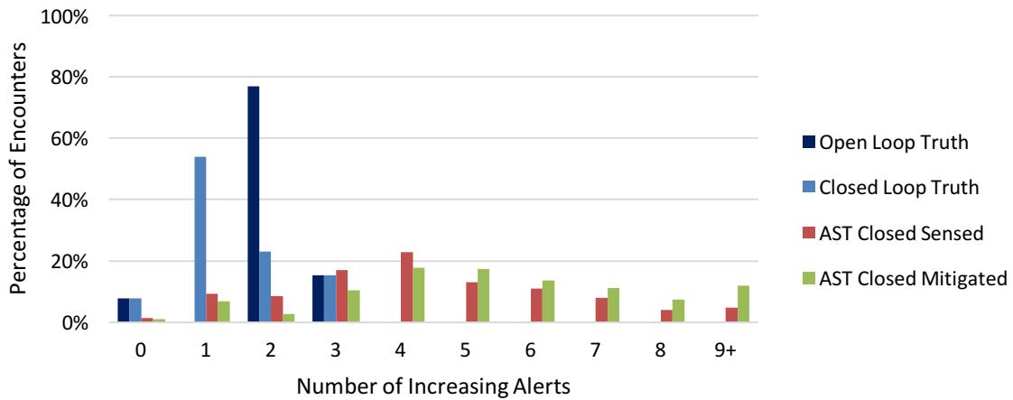
Figure 92. AST Alert Jitter for Converging MOPS Requirement-Derived Test Vectors
