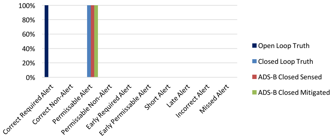
Figure 70. ADS-B Corrective Alert Scoring for High Speed MOPS Requirement-Derived Test Vectors
