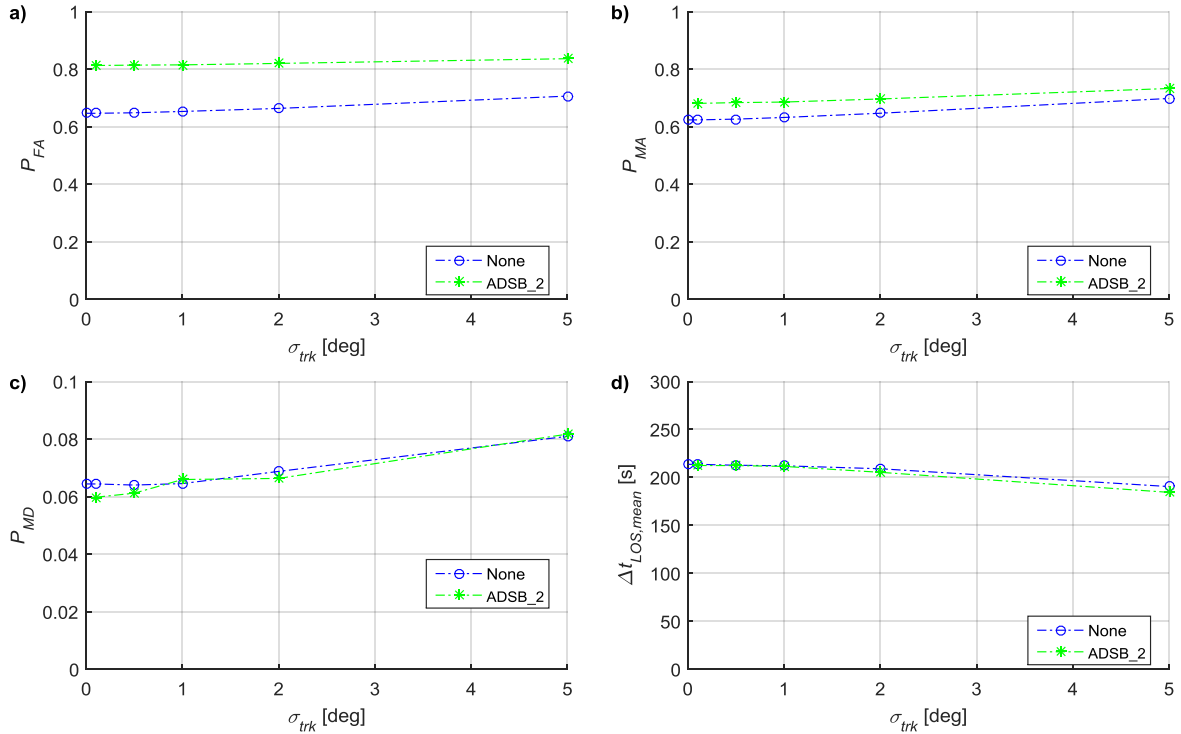
Figure 38. CD performance metric sensitivities to surveillance track angle error standard deviation with no other surveillance error (None) and with the ADSB_2 surveillance error model.
