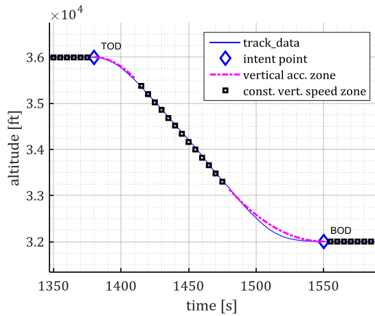
Figure 12. Example identified vertical intent points with vertical acceleration zones and constant vertical speed segments.
