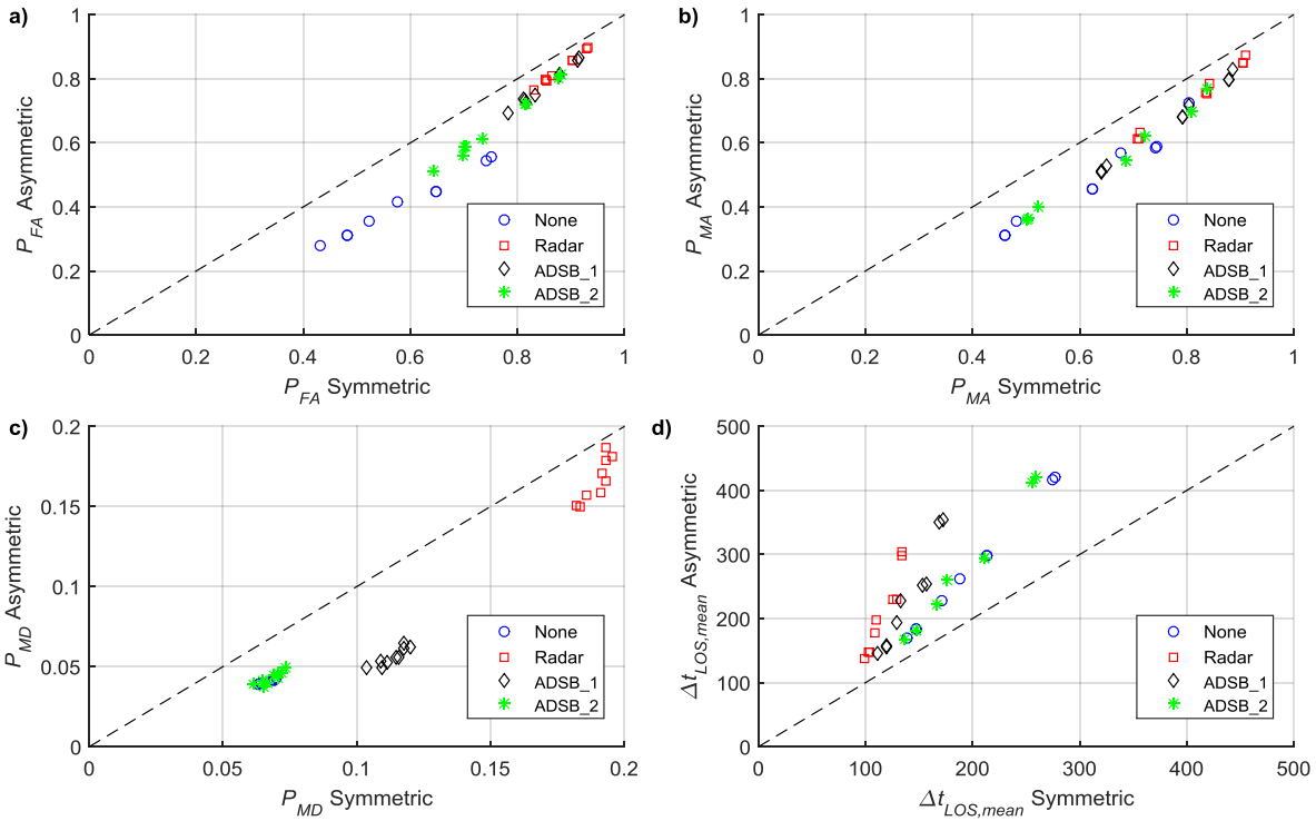
Figure 29. Difference in CD performance metrics between symmetric and asymmetric trajectory predictions over all SQ1 surveillance quality analysis runs with CD cycle period of 60 seconds.
