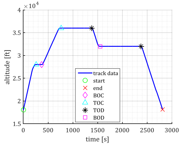
Figure 10. Sample recorded track vertical profile with identified altitude change points.
