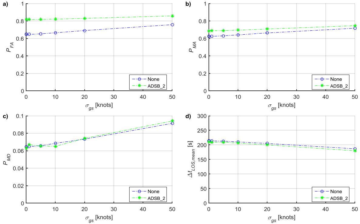
Figure 36. CD performance metric sensitivities to surveillance groundspeed error standard deviation with no other surveillance error (None) and with the ADSB_2 surveillance error model.
