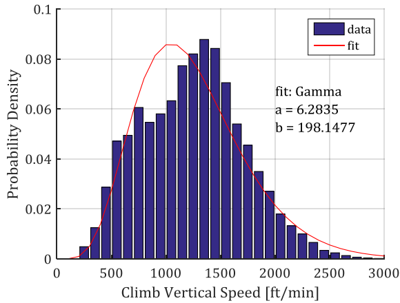
Figure 20. Distribution of the average vertical speed between vertical level segment changes in climbs for all tracks.
