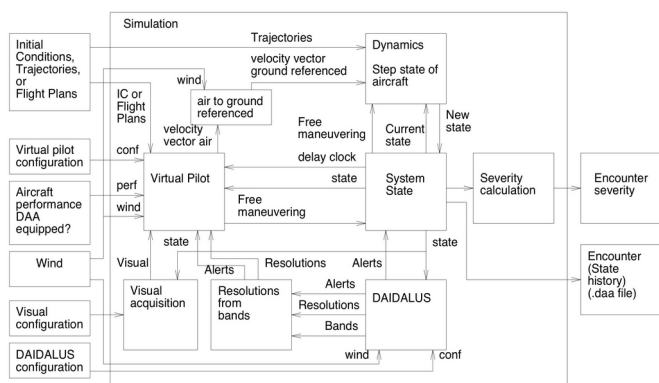
Fig 4. Fast-time simulation functional diagram
