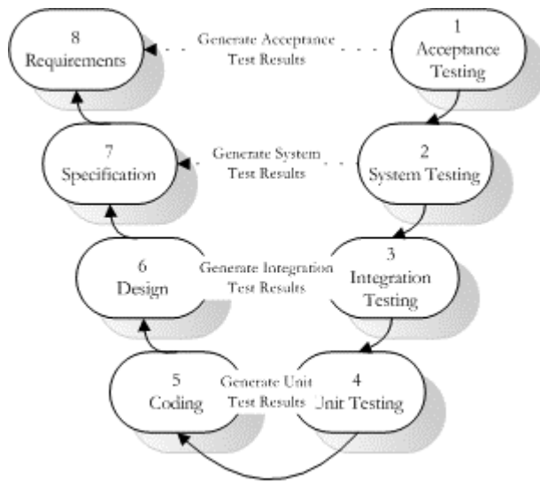
Figure 1.2 - Reverse V-Model
